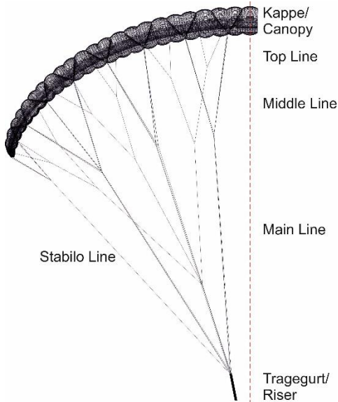
Fig. 1 CAD drawing of ARCUS RS
